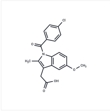
Chemical structure of Indomethacin(吲哚美辛)(COX 抑制 剂),CAS No.53-86-1
