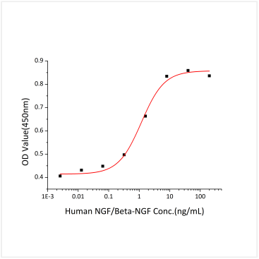
Measured in a cell proliferation assay using TF-1 Human erythroleukemic cells. The ED 50 for this effect is 0.58-2.35 ng/mL, corresponding to a specific activity of 4.25×10 5 ~1.70×10 6 units/mg.
