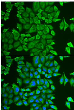
Immunofluorescence analysis of HeLa cells using APEH antibody (A13467). Blue: DAPI for nuclear staining.
